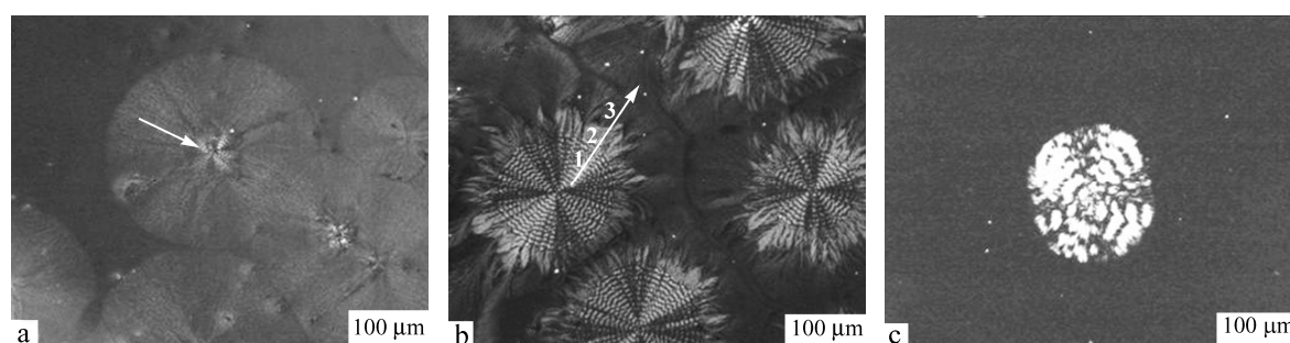
Fig. 1 Optical micrographs showing the morphologies of (a) neat PVDF crystallized isothermally at 170°C, (b) the PVDF in a 70/30 PVDF/PBS blend crystallized isothermally at 167°C and (c) the PVDF in a 30/70 PVDF/PBS blend crystallized isothermally at 167°C for 100 h
