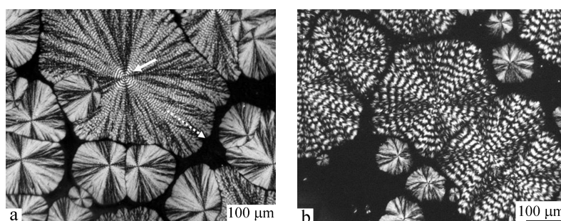
Fig. 4 Optical micrographs of PVDF in (a) 70/30 PVDF/PBS blend crystallized completely at 162°C and (b) 30/70 PVDF/PBS blend crystallized at 162°C for 100 h
